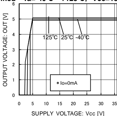
Fig.2 Line Regulation
