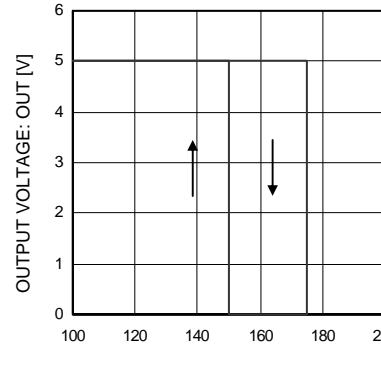
Fig.12 Thermal Shut Down
