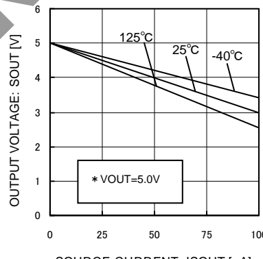
Fig.10 SOUT Pull Up Resistor
