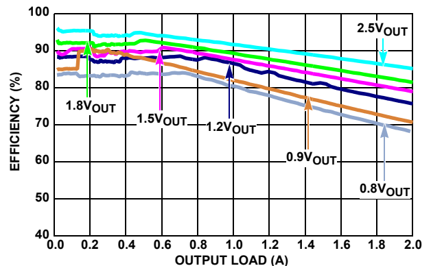
FIGURE 2. EFFICIENCY vs LOAD ( f_{SW} = 2\text{MHz} , V_{IN} = 3.3\text{V} , MODE = PFM, T_A = +25^\circ\text{C} )
