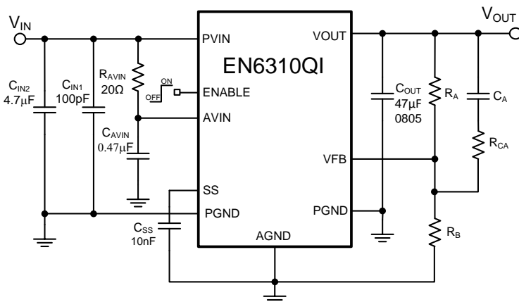
Figure 1. Simplified Applications Circuit
