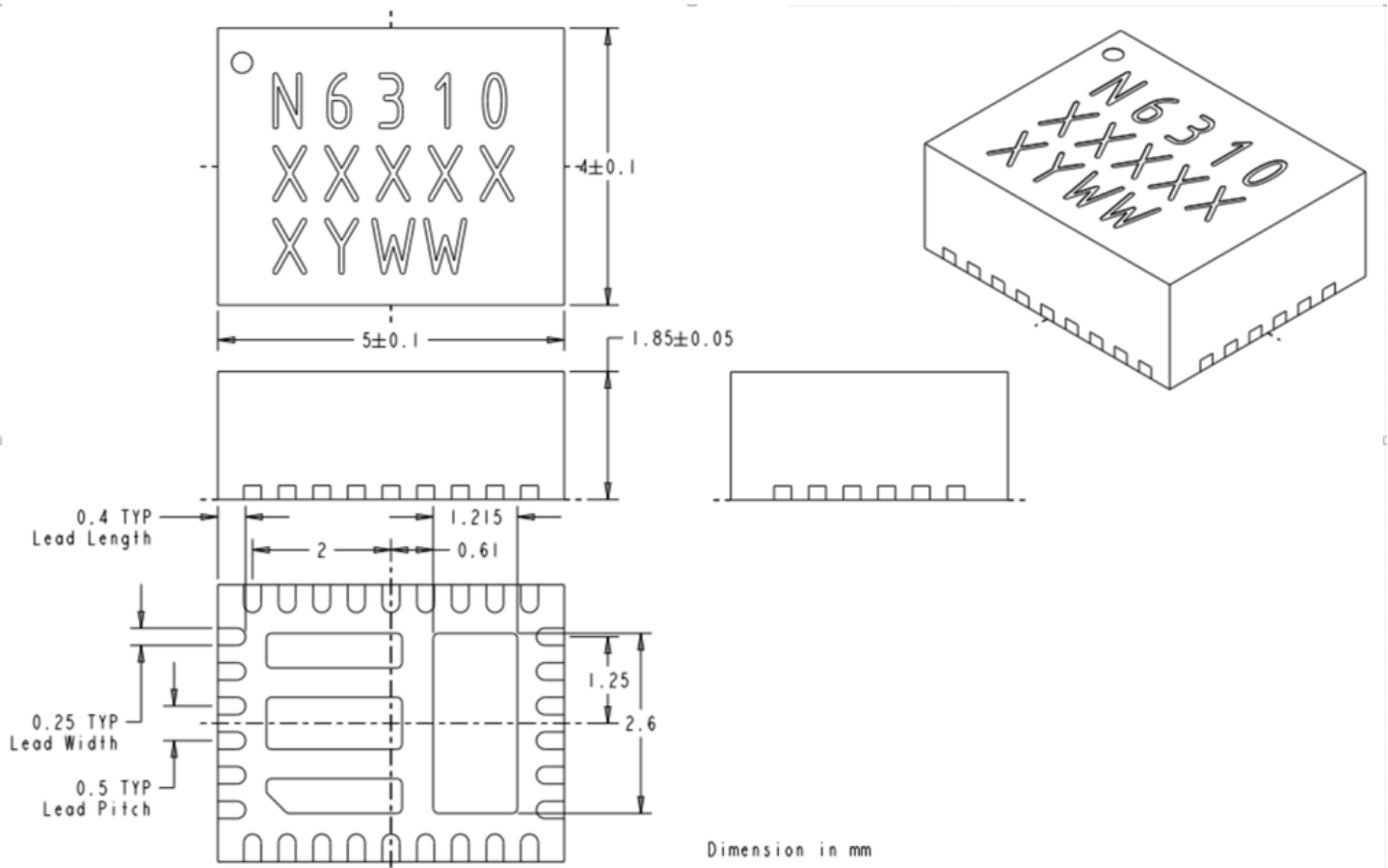
Figure 10. EN6310QI Package Dimensions (Bottom View)
