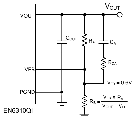
Figure 5. External Compensation
