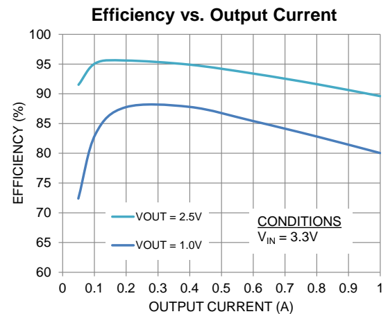
Figure 2. Highest Efficiency in Smallest Solution Size
