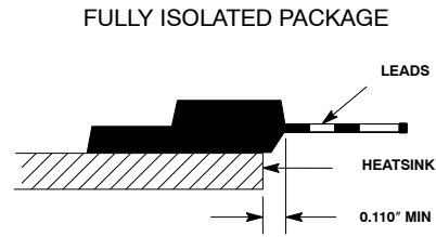
Figure 14. Mounting Position
