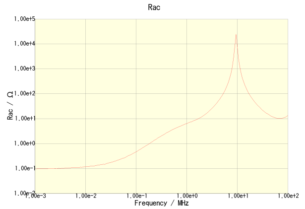
CLF6045T-330M-CA
