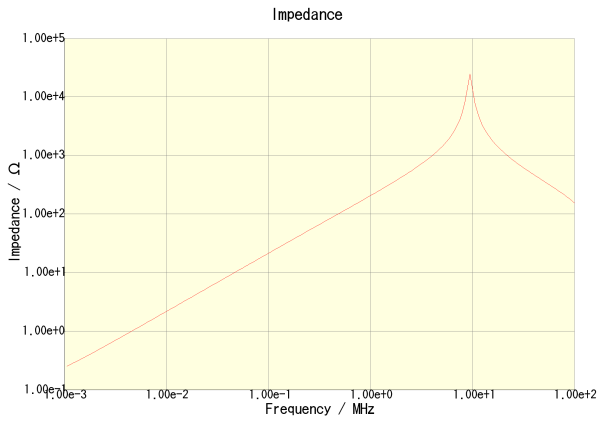
CLF6045T-330M-CA
