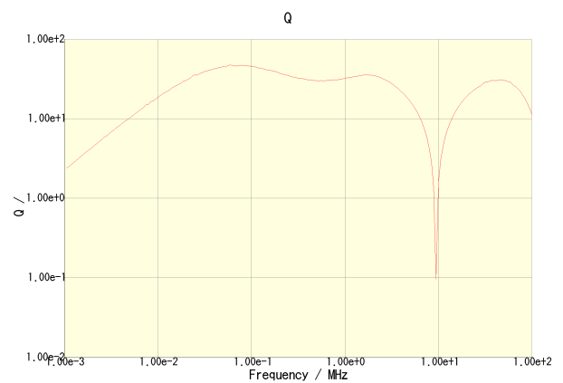
CLF6045T-330M-CA
