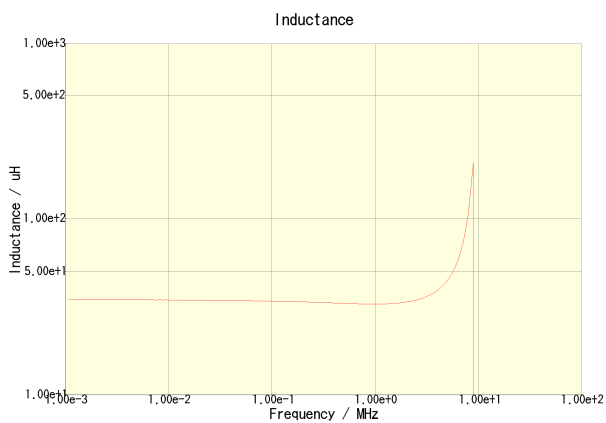
CLF6045T-330M-CA
