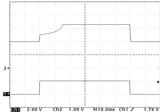
Figure 20. Startup Transient Response Upper Trace: Output Voltage Waveform, 2.0 V/Division Lower Trace: Shutdown Pin Waveform, 1.0 V/Division
